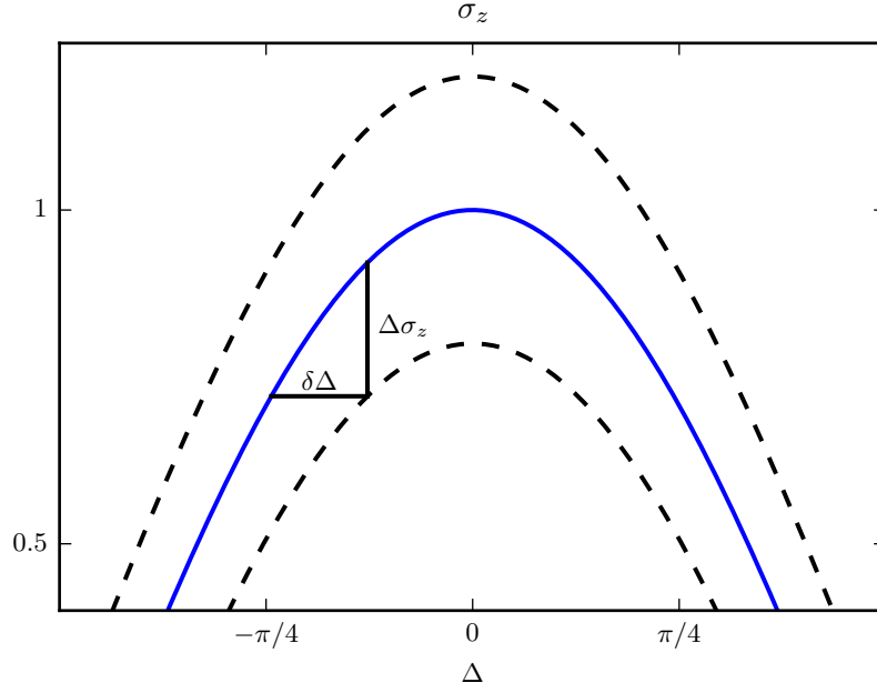
Figure 3.7: Illustration of the meaning of the signal sensitivity \delta\Delta . The solid blue curve depicts the signal \langle \sigma_z \rangle , while the two dashed curves illustrate the signal boundaries in the sense of its rms deviation. At any chosen point the sensitivity can be extracted from the slope triangle between the signal curve and signal plus/minus its rms deviation.
