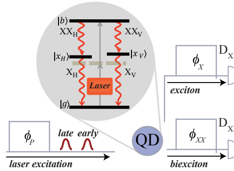
Figure 12.1: (Colour online) Schematic of time-bin entanglement. The quantum dot system (QD) is excited by two consecutive pulses obtained from an unbalanced Michelson interferometer shown on the left. The relative phase between these pulses is \phi_P . The state analysis is performed using additional two interferometers, one for the exciton and the other for the biexciton photons. These two interferometers have their respective phases, \phi_X and \phi_{XX} . The photons are detected upon leaving the analysis interferometers using detectors D_X and D_{XX} . The level scheme depicts the quantum dot excited resonantly from the ground state |g\rangle to the biexciton state |b\rangle using a two-photon excitation. A pulsed laser populates the biexciton via a virtual level (dashed grey line). The system decays emitting a biexciton-exciton photon cascade ( XX_V and X_V or XX_H and X_H ).
