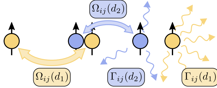
Figure 11.1: (Colour online) Scheme of a 2D optical lattice filled with clock atoms interacting via dipole-dipole energy exchange \Omega_{ij} and a collectively modified spontaneous emission \Gamma_{ij} at two different lattice constants shown in blue and yellow. In a mean field treatment with translation invariance the sum over all interaction terms yields two effective couplings \Omega^{\text{eff}} and \Gamma^{\text{eff}} only, which govern the approximate system dynamics.
