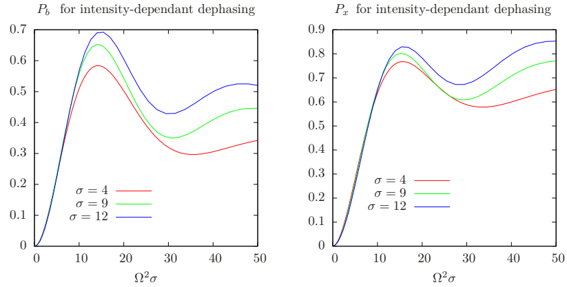
Figure 12.7: Rabi oscillations for linearly intensity-dependent dephasing with an amplitude of \gamma_{I_0} = 0.05 as a function of the deposited energy. The emission probability from the biexciton (left) and the exciton (right) level is shown. From this it is clear that the ratio between the first Rabi maximum and its first minimum is largely determined by \gamma_{I_0} . The figure for n_p = 4 looks fairly similar and is therefore omitted.
