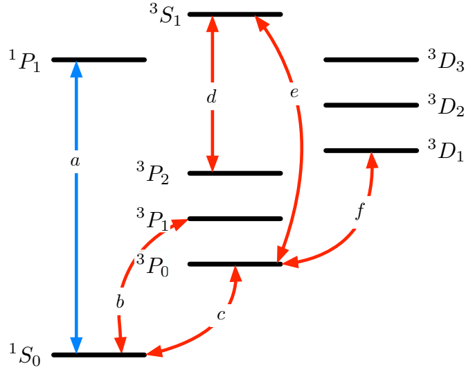
Figure 3.4: Simplified level structure of ^{87}\text{Sr} . In the outer-most orbitals various transitions are involved in cooling and trapping the atoms. The transition ^1S_0 \rightarrow ^3P_0 (c) is the actual clock transition. For details see tbl. 3.2.
