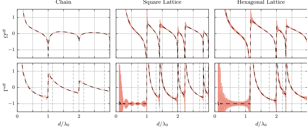
Figure 11.3: (Colour online) Distance dependence of the effective quantities \Omega^{\text{eff}} and \Gamma^{\text{eff}} for an infinite equidistant chain, a square lattice and a hexagonal lattice (dashed black) compared to their not yet converged finite counterparts of 10 , 4 \cdot 10^4 and 10^5 particles respectively (solid red). Again, we find divergences at integral d/\lambda_0 owing to the 1/\xi -terms in F(\xi) and G(\xi) . In the 2D configurations \Gamma^{\text{eff}} plateaus at -1 for d < \lambda_0 , suggesting that this parameter range will be the most favourable for clock setups as decay is strongly suppressed. Finite sample sizes in our numerics can lead to strong oscillations of the effective quantities at small distances and even to unphysical values of \Gamma^{\text{eff}} < -1 .
