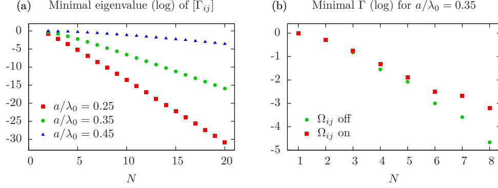
Figure 7.5: Subradiant behaviour for increasing N . a) Minimum decay rate (or eigenvalue) obtained from [\Gamma_{ij}] with increasing atom number N in a linear chain configuration for different spacings a . Smaller distances show a close to exponential and drastic decrease of \Gamma_{\min} with increasing N . b) Scaling of the \Gamma_{\min} obtained via the population accumulation method (as detailed in the text) with and without coherent dipole-dipole energy exchange.
