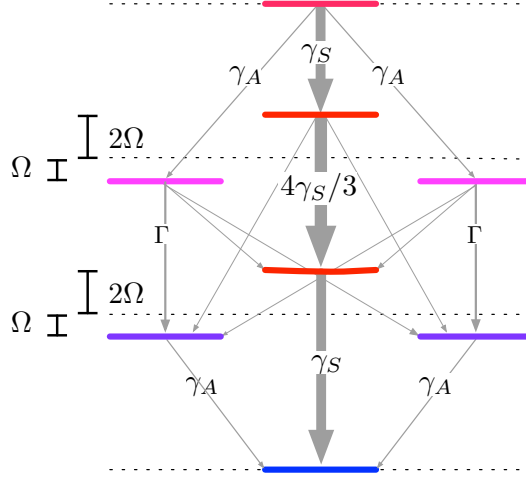
Figure 7.3: Energy levels and decay channels for three equidistant atoms. Results of the diagonalization of both the Hamiltonian and the Liouvillian for three atoms in an equidistant triangle configuration. The dipole-dipole shifts of levels are depicted with the corresponding decay channels and rates. Further details can be found in Ref. [144].
