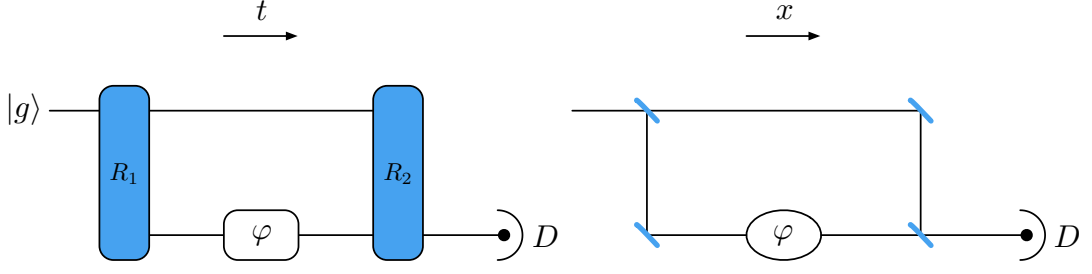
Figure 3.5: Illustration of the Ramsey interferometry procedure. In comparison to a Mach-Zehnder interferometer in classical optics (right). In a Ramsey procedure (left) the interference fringes are created by a phase imprinted on the coherence between |g\rangle and |e\rangle , while in a classical interferometric experiment the interference pattern stems from combining the two split up fields of different optical path lengths again before detection.
