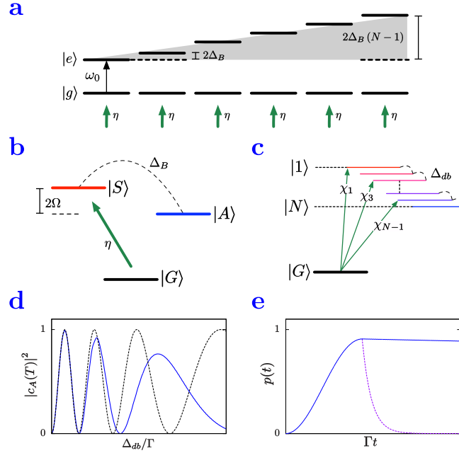
Figure 8.2: Coupling to dark states via a magnetic field gradient. a) Linearly increasing level shifts along the chain occurring in the presence of the magnetic field gradient. b) Illustration of the level structure and indirect dark state access for two coupled emitters. While symmetry selects the state |S\rangle , off-resonant addressing combined with bright-dark state coupling of strength \Delta_B allows for a near-unity population transfer into the state |A\rangle . c) Dynamics in the single-excitation manifold of N coupled emitters where symmetric driving reaches the bright states with amplitudes \chi_m while the magnetic field couples neighbouring dark and bright states. d) Plot of the asymmetric state population for the two-atom case as a function of the increasing magnetic field (solid line) compared to the steady-state approximation (dashed line) at numerically optimized time T = 16.19 \Gamma^{-1} , with parameters \eta = \Gamma and a = 0.05 \lambda_0 . e) For a chain of N = 4 emitters, a 91%-efficient \pi -pulse to the most robust state can be achieved as demonstrated in the population evolution plot. The separation is chosen to be a = 0.025 \lambda_0 , while \eta = 40 \Gamma and numerical optimization is employed to find \Delta_B = 0.98 \Gamma .
