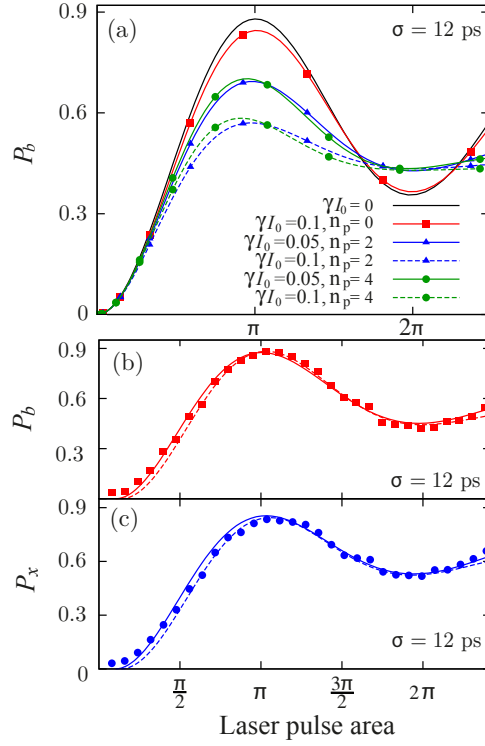
Figure 12.3: (Colour online) a) Biexciton emission probability, P_b (theory) for different dephasing models. We observe a strong damping of the Rabi oscillations even at moderate \gamma I_0 . From this it is clear that the amplitude of the intensity-dependant dephasing rate plays a much greater role than the exponent n_p . b) Emission probability for a biexciton, P_b , and exciton photon, P_x , as a function of the laser pulse area for linear (solid line) and quadratic (dashed line) intensity-dependent dephasing compared to the experimental data, respectively. The error bars are smaller than symbols. The theoretical parameters, \gamma I_0 , are obtained by fitting the ratio of the first maximum and minimum of the Rabi cycle.
