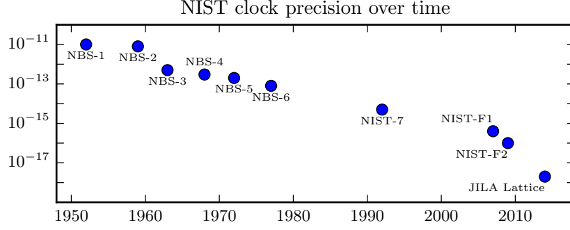
Figure 3.3: Overview of atomic clock precision at NIST/JILA. Qualitatively, an almost exponential increase in precision can be observed. (Almost) all of these clocks have served as primary frequency standards. Data due to NIST/JILA [59, 74].
