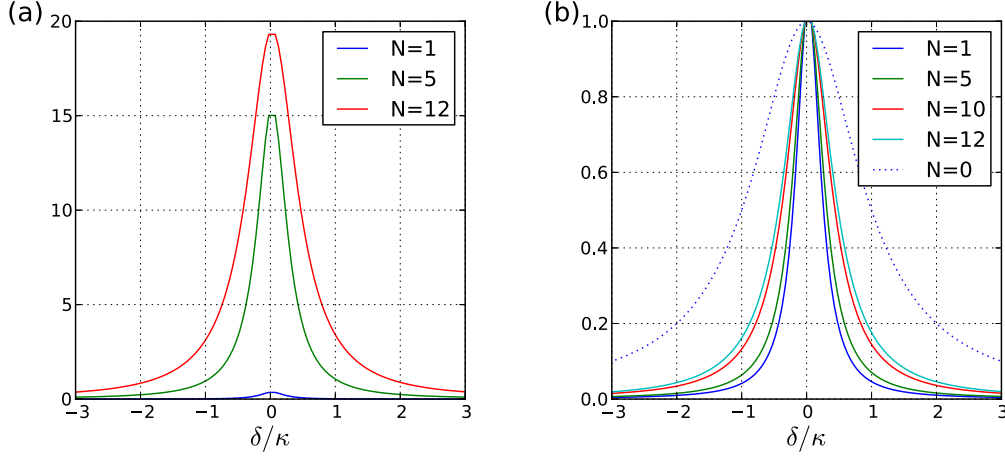
Figure 9.3: Output spectrum of a fully collective laser with different atom numbers N for \Gamma = \kappa/20 and R = \kappa/5 compared to the empty cavity linewidth ( N = 0 ), absolute (a) and normalized (b).
