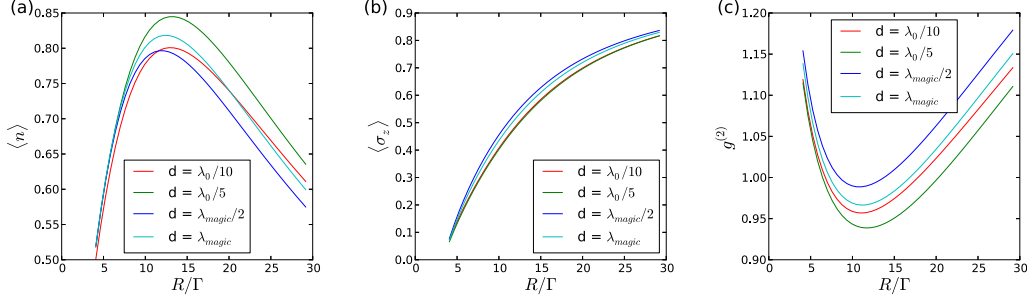
Figure 9.6: Photon number (a), atomic inversion (b) and g^2 function (c) of the laser as a function of the pump strength R for a square of different lattice constants d and a fixed spontaneous decay rate \Gamma = 0.2\kappa .
