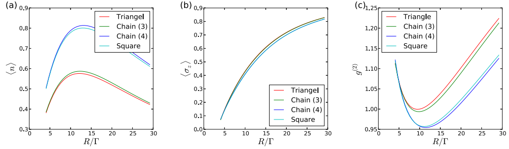
Figure 9.5: Photon number (a), atomic inversion (b) and g^{(2)} function (c) of the laser as a function of the pump strength R for different atomic arrangements and a fixed spontaneous decay rate \Gamma = 0.2\kappa .
