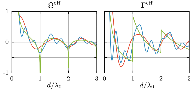
Figure 11.2: (Colour online) Distance dependence of the effective dipole coupling \Omega^{\text{eff}} and \Gamma^{\text{eff}} for a square (red), a ten-sided (blue) and a 100000-sided (green) regular polygon. The fewer particles the closer the functions resemble the underlying couplings \Omega_{ij} and \Gamma_{ij} . The divergences at integral d/\lambda_0 result from the 1/\xi terms in F(\xi) and G(\xi) .
