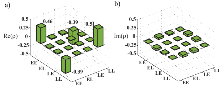
Figure 12.5: (Colour online) An example of (a) real and (b) imaginary part of the reconstructed density matrix. Measurements used to obtain this density matrix were performed using 12 ps excitation pulses while the emission probability was kept at 6%. Here, E (early) and L (late) denote the measurement basis.
