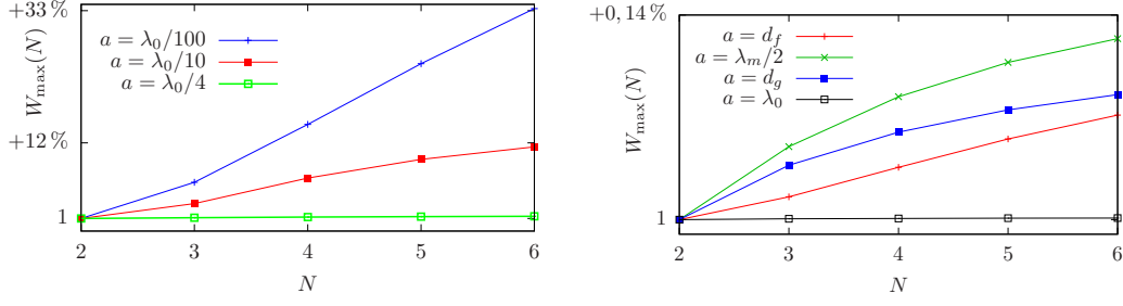
Figure 5.7: Maximum of the energy emission as a function of the number of atoms in the chain for small (left) and large (right) lattice constants a . The distances d_f and d_g refer to the first root of the functions F and G , respectively.
