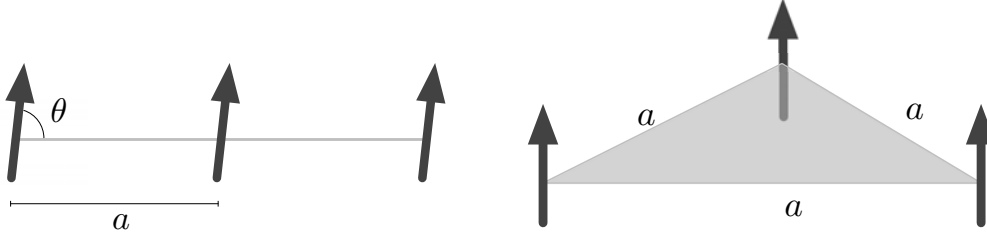
Figure 5.3: Linear chain and triangular array of three atoms with lattice constant a and angle \theta .
