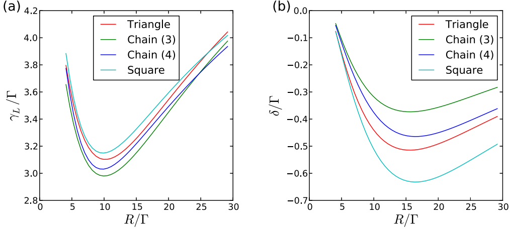
Figure 9.8: Laser linewidth (a) and frequency shift (b) for different geometric configurations but same lattice constant ( d = \lambda_0/10 ) as a function of the pump strength for a fixed atomic decay rate of \Gamma = 0.2\kappa .
