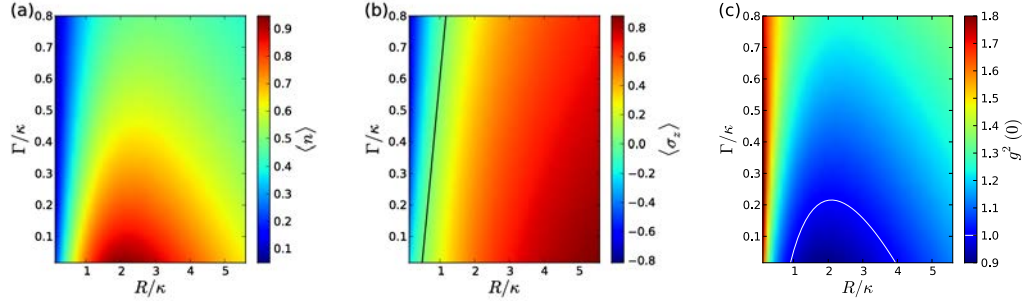
Figure 9.4: Stationary operation of a four atom laser on a square lattice. (a) photon number, (b) atomic inversion, where the black line indicates equal population of the excited and the ground state, (c) g^{(2)}(0) function, with the white line at g^{(2)}(0) = 1 representing a coherent state.
