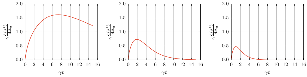
Figure 11.9: Slope of the signal at the zero crossing of the first fringe after a free evolution time of \gamma t for different sets of effective interaction strengths as above, from left to right: ( \Omega^{\text{eff}} = 0, \Gamma^{\text{eff}} = -0.75 ), ( \Omega^{\text{eff}} = 0, \Gamma^{\text{eff}} = 0 ) and ( \Omega^{\text{eff}} = 1, \Gamma^{\text{eff}} = 1 ).
