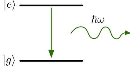
Figure 4.1: Spontaneous emission. A two-level quantum system decays from the excited state |e\rangle to the ground state |g\rangle and emits a photon of the energy \hbar\omega = E_e - E_g with random polarization into a random direction.
