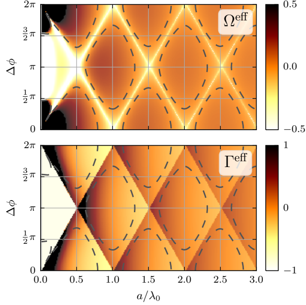
Figure 11.4: (Colour online) Effective interactions \Omega^{\text{eff}} and \Gamma^{\text{eff}} for an infinite chain with spacing a where the spins are initially prepared with phase shift \Delta\phi between neighbouring spins. The dashed lines indicate parameters with \Omega^{\text{eff}} = 0 optimal for an optical clock.
