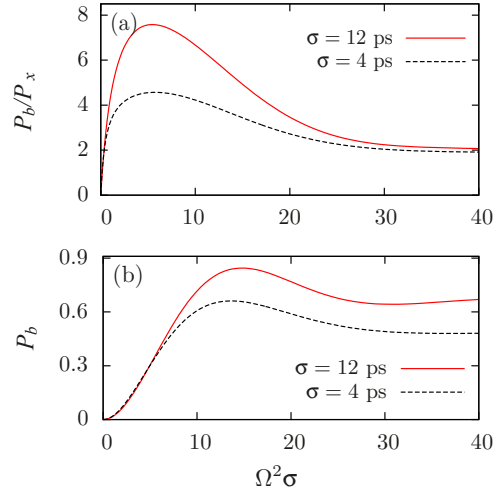
Figure 12.4: (Colour online) Relative probability for biexciton versus single exciton excitation in the quantum dot as a function of \Omega^2\sigma for two different pulse lengths (upper plot). The choice of \Omega^2\sigma , which is proportional to the energy per pulse, as x-axis allows for easier comparison of the maxima. We see an optimum ratio of about 8 at a still moderate excitation rate. The lower plot gives the biexciton photon emission probability as a function of \Omega^2\sigma .
