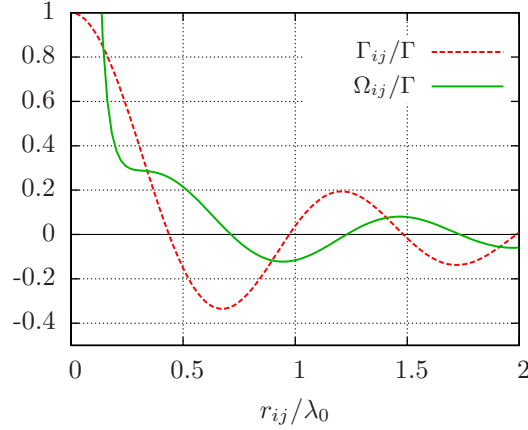
Figure 5.1: Collective spontaneous emission \Gamma_{ij}/\Gamma and resonant dipole-dipole coupling \Omega_{ij}/\Gamma for \theta = \pi/2 as a function of inter-atomic distance in units of the resonant wavelength \lambda_0 .
