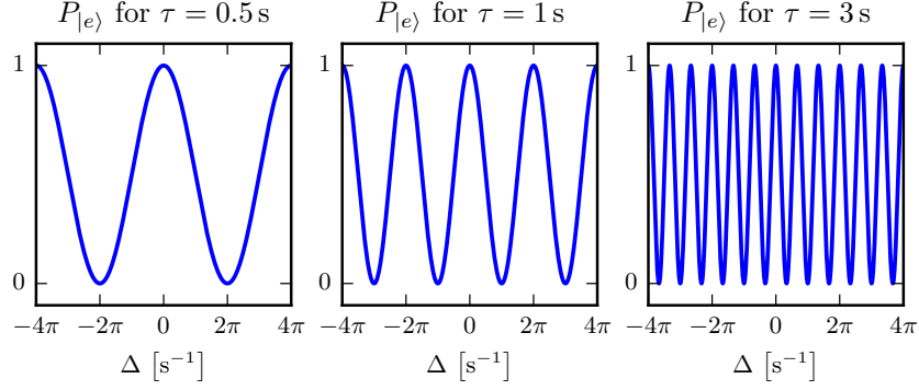
Figure 3.6: Ramsey fringes for different interrogation times \tau . The longer the probing time, the closer the fringe spacing, which increases the discernibility or resolution of the individual fringes.
