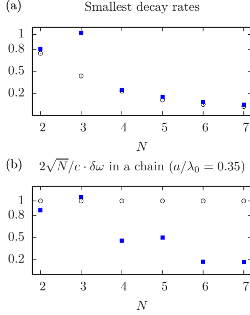
Figure 7.6: Scaling laws. a) Scaling of the extrapolated inverse timescale 2/\tau_{\text{opt}} with increasing N (squares) compared to the theoretical scaling of \Gamma_{\text{min}} (circles). b) Scaling of the minimum sensitivity (times 2\sqrt{N}/e ) obtained via PRT with particle number (always for the PRT with m = \lfloor N/2 \rfloor ). The circles show the normal scaling of SRT on independent atoms 2\sqrt{N}/e \cdot \delta\omega = 1 . For an even particle number, the rotation with m = N/2 corresponds to a configuration where the system is composed of non-radiative atom pairs. For odd particle number, there is one unpaired spin and the resulting sensitivity is roughly the one obtained for N - 1 atoms (except for small systems where the effect of the unpaired atom is substantial).
