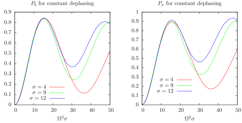
Figure 12.6: Rabi oscillations for constant dephasing as a function of \Omega^2\sigma . The emission probability for the biexciton, P_b , (left) and the exciton, P_x , (right) level are shown. It is obvious that short pulses introduce damping of the Rabi oscillations.
