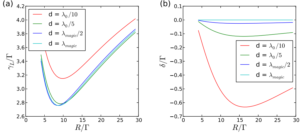
Figure 9.7: Laser linewidth (a) and frequency shift (b) for a square atom arrangement at different distances as a function of the pump strength for a fixed atomic decay rate of \Gamma = 0.2\kappa .
