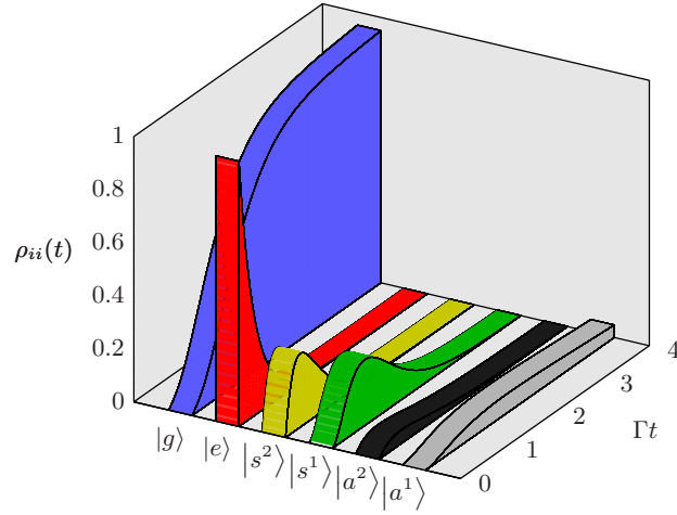
Figure 5.5: Decay from the fully inverted state via |s^2\rangle , |a^2\rangle (and |b^2\rangle , which due to the degeneracy shows the same behaviour) and the single-excitation states |s^1\rangle and |a^1\rangle (and |b^1\rangle ) to the ground state for \gamma = 0.71\Gamma ( a = \lambda_0/5 ).
