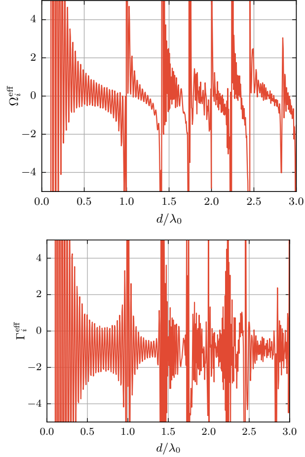
Figure 11.6: Effective quantities \Omega_i^{\text{eff}} and \Gamma_i^{\text{eff}} as experienced for the innermost spin inside a cube consisting of 2001 \times 2001 \times 2001 spins in a cubic lattice configuration depending on the lattice spacing d . Even for very small changes of the lattice spacing the mean net-effect of all other spins will change dramatically. Unphysical values of \Gamma^{\text{eff}} < -1 emerge due to numerical artifacts and too slow a convergence.
