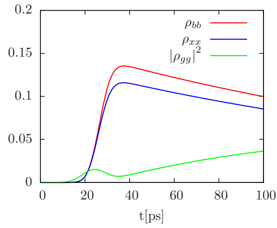
Figure 12.8: Time evolution of exciton \rho_{xx} and biexciton \rho_{bb} population as well as the biexciton-ground coherence as a function of time for a Gaussian pulse of \sigma = 12 ps.
