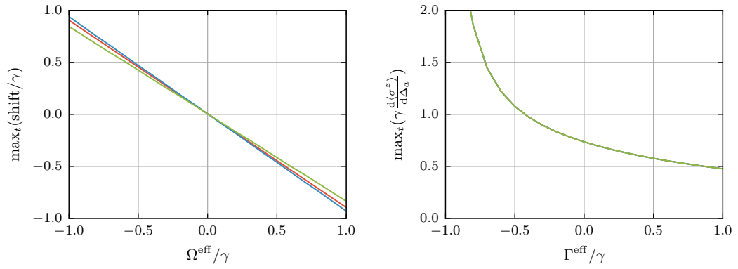
Figure 11.10: (a) Shift of Ramsey fringes depending on the effective coupling \Omega^{\text{eff}} after t = 15\gamma^{-1} . The different lines represent different choices of \Gamma^{\text{eff}} , which hardly influence the result. The fringe shifts follow the effective mean field dipole coupling \Omega^{\text{eff}} almost linearly and thus can be read off from the figures in the main manuscript. (b) Maximally achievable slope at roots depending on \Gamma^{\text{eff}} . The result is independent of the choice of \Omega^{\text{eff}} . Note that a negative \Gamma^{\text{eff}} improves the measurement precision beyond the independent atom value.
