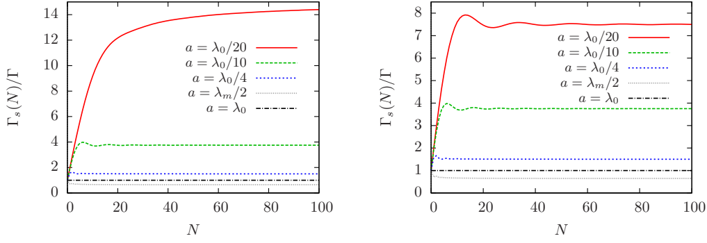
Figure 5.2: Symmetric exciton state decay rate \Gamma_s(N)/\Gamma as function of atom number for \theta = 0 (left) and \theta = \pi/2 (right).
