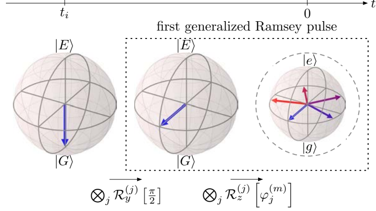
Figure 7.2: Phase-spread operation. Redesign of the first Ramsey pulse to include, in addition to the initial \pi/2 pulse, rotations of the individual spins with different angles such that the resulting overall dipole moment vanishes. Notice that the last Bloch sphere has a radius 1/2 , corresponding to single spins.
