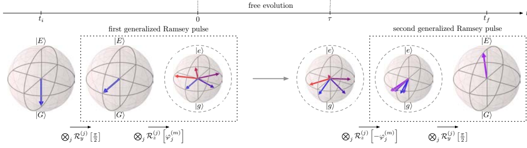
Figure 6.1: State protective Ramsey sequence. The ensemble of N spins starts with all spins down in a collective coherent pure spin state on the surface of the collective Bloch sphere (radius N/2 ). Individual \pi/2 pulses are followed by phase encoding operations of angles \varphi_j^{(m)} = (2\pi m/N)(j-1) where j = 1, \dots, N and m = 1, \dots, [N/2] , which brings the total spin close to the centre of the Bloch sphere (third-fifth steps are shown on small Bloch spheres of radius 1/2 ). After time \tau , the phase encoding operation is reversed and \pi/2 pulses prepare the ensemble (now in a mixed state shown on the large collective Bloch sphere) for the detection of the population difference signal.
