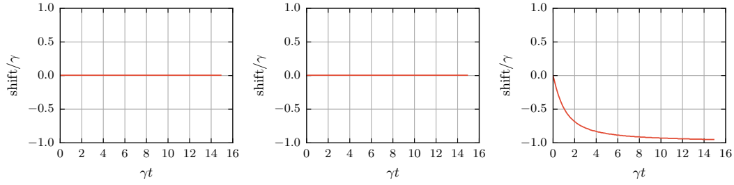
Figure 11.8: Shifts of the maxima after the free evolution time \gamma t for different sets of effective interaction strengths as above, from left to right: ( \Omega^{\text{eff}} = 0, \Gamma^{\text{eff}} = -0.75 ), ( \Omega^{\text{eff}} = 0, \Gamma^{\text{eff}} = 0 ) and ( \Omega^{\text{eff}} = 1, \Gamma^{\text{eff}} = 1 ).
