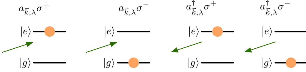
Figure 4.2: Processes involved In dipole-approximation there are four processes that can occur, when a two-level atom interacts with a field. Two of them are energy-conserving and are kept in the rotating wave approximation, while the other two are dropped, as discussed in the text.
