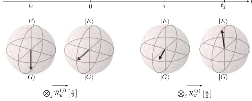
Figure 7.1: Standard Ramsey metrology. The ensemble of N spins starts with all spins down in a collective coherent pure spin state on the surface of the collective Bloch sphere (radius N/2 ). The first \pi/2 pulse aligns the average collective dipole along the x axis and free evolution is allowed. After the interrogation time \tau , another \pi/2 pulse follows which attempts to align the state with the excited state and fails by an angle that depends on the accumulated phase during free evolution as well as on the total decay of the collective state. The detected signal to be analyzed is a measure of population inversion.
