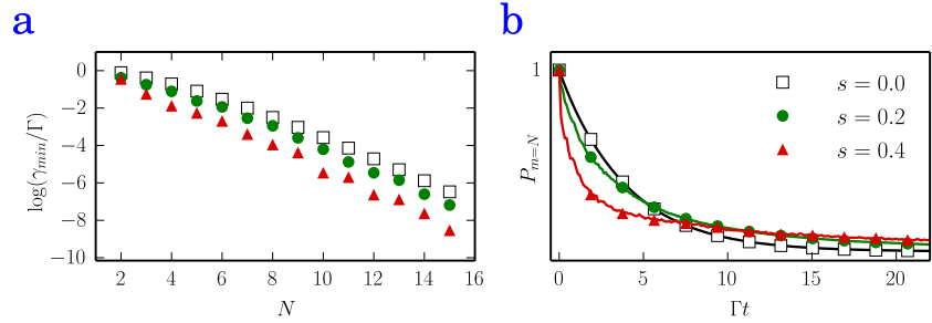
Figure 8.4: Subradiance and disorder. a) Plot of the logarithm of the minimal eigenvalue of the decay rate matrix (matrix with entries \gamma_{ij} ) as a function of N at a distance of a = 0.4\lambda_0 for increasing levels of disorder ( s = 0, 0.2, 0.4 ). b) Decay of the |m = N\rangle state as a function of time. In the presence of disorder ( s = 0.2, 0.4 ) the short time and long time behaviours are fundamentally different. At short times, disorder can push the state towards faster decaying channels while decay inhibition due to disorder occurs at larger times.
