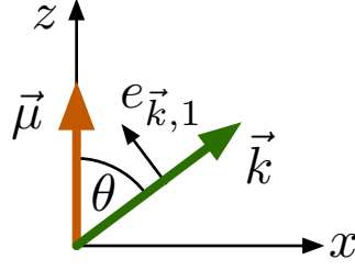
Figure 4.3: Angles between \vec{k} and \vec{\mu} . This figure visualizes the resolution of the polarization sum of eq. (4.16).
