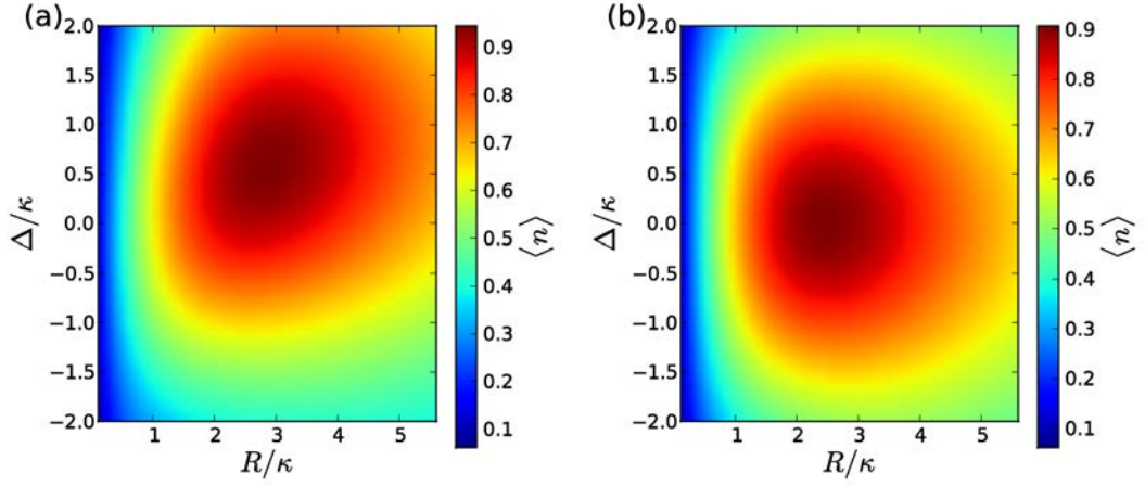
Figure 9.9: Average photon number for atoms on a square with d = \lambda_0/10 (a) and d = \lambda_{\text{magic}}/2 (b) for variable cavity detuning and an atomic decay rate \Gamma = 0.2\kappa .
