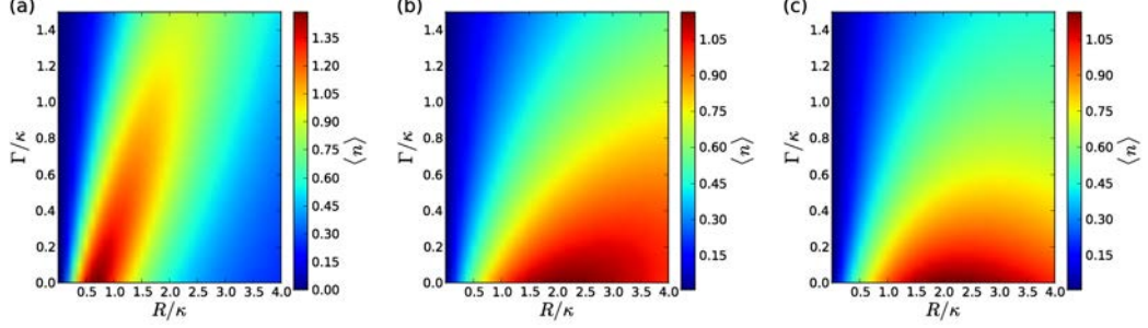
Figure 9.2: Stationary photon number as a function of the pump strength R and the spontaneous decay rate \Gamma for collectively pumped and collectively decaying atoms (a), individually pumped but collectively decaying atoms (b) and individually pumped and individually decaying atoms (c).
