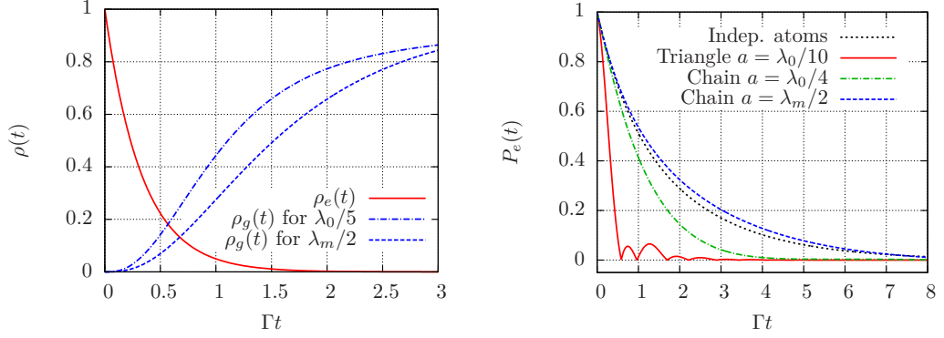
Figure 5.6: Collective decay from fully excited state to the ground state in the equilateral triangle for a = \lambda_0/5 and a = \lambda_m/2 (left) and its influence on the maximal Ramsey signal contrast for independent atoms, atoms closely positioned in a triangle as well as in a chain (green) and at magic wavelength-distance (right).
