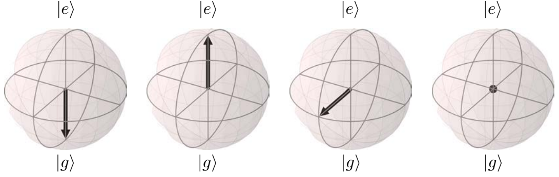
Figure 2.1: Example of Bloch spheres. Their south pole represents the ground state |g\rangle and their north pole the excited state |e\rangle . The visualized states (from left to right) are the three pure states |g\rangle , |e\rangle and 1/\sqrt{2}(|g\rangle + |e\rangle) as well as the mixed state |e\rangle\langle e| + |g\rangle\langle g| .
