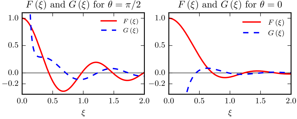
Figure 4.4: Dissipative and coherent couplings F(\xi) and G(\xi) . Here, \xi = r_{ij}/\lambda_0 and \lambda_0 = 2\pi/k_0 , i.e., we have scaled the arguments with a factor of 2\pi for the plots.
