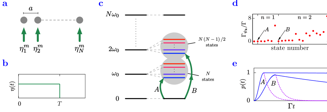
Figure 8.1: Selective state preparation procedure. a) A chain of N closely spaced quantum emitters (separation a with ka \ll 1 , k being the laser wave number) are individually driven with a set of pumps \{\eta_j^m\} . b) The lasers are turned on for a time T , optimized such that an effective \pi -pulse into the desired subradiant target state is achieved. c) Level structure for the N systems where the C_n^N -fold degeneracy of a given n -excitation manifold is lifted by the dipole-dipole interactions. The target states are then reached by energy resolution (adjusting the laser frequency) and symmetry (choosing the proper m ). d) Scaling of the decay rates of energetically ordered collective states starting from the ground state (state index 1) up to the single- and double-excitation manifolds for 6 particles at a distance of a = 0.02 \lambda_0 . The arrows identify the decay rates for the lowest energy states in the single (A) and double (B) excitation manifolds. e) Numerical results of the time evolution of the target state population for N = 6 and a = 0.02 \lambda_0 during and after the excitation pulse. Near unity population is achieved for both example states A (where we used \eta = 0.53 \Gamma ) and B (for \eta = 2.44 \Gamma ) followed by a subradiant evolution after the pulse time T shown in contrast to the independent decay with a rate \Gamma (dashed line).
