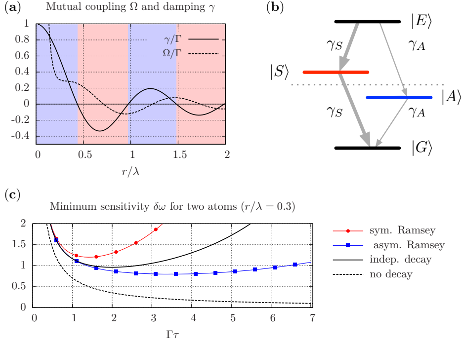
Figure 6.2: Two atoms metrology. (a) Normalized mutual decay rate and dipole-dipole frequency shift for a pair of atoms as a function of r/\lambda . For positive/negative \gamma , the asymmetric state is subradiant/superradiant (indicated by the colour-coded regions). (b) Level scheme in the dressed basis showing the two independent decay channels with modified rates \gamma_S and \gamma_A . (c) Optimal sensitivity as a function of \tau\Gamma . The atom separation is r/\lambda = 0.3 corresponding to \gamma \approx 0.41 \Gamma and \Omega \approx 0.29 \Gamma . The minimum for the asymmetric addressing is reached around \tau \simeq 2/\gamma_A .
