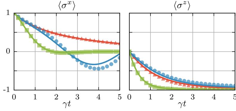
Figure 11.5: (Colour online) Three different examples for the time evolution of the spin expectation values for a chain with spacing d where initially all spins are prepared in a coherent superposition of ground and excited state with a phase shift of \Delta\phi . The parameters used are d = 0.792\lambda_0 with \Delta\phi = 0 (red triangles), where \Omega^{\text{eff}} = 0 and \Gamma^{\text{eff}} is nearly optimal, as well as d = 0.49\lambda_0 (green squares) and d = 0.51\lambda_0 (blue circles), both with \Delta\phi = \pi which are close to a \Gamma^{\text{eff}} discontinuity. The solid lines correspond to a solution of a second order cumulant expansion model with 200 particles and demonstrate a very good agreement with the infinite mean field description.
