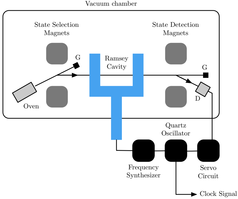
Figure 3.1: Schematic of a beam-based atomic clock. The atoms are heated up in the oven, those with the desired internal state are directed into the interrogation region, where they pass through the Ramsey cavity. Another set of magnets prepares the atoms which have flipped their state for being counted at the detector (D). In both sets of magnets about half of the passing atoms are lost and collected by the getter (G). The servo circuit optimizes the frequency of the cavity, which is generated by a Quartz oscillator and modulated by the frequency synthesizer so that the maximum number of atoms will be counted. A clock signal can be derived from the Quartz oscillator.
