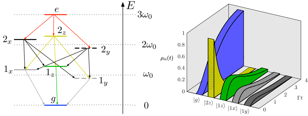
Figure 5.4: Decay scheme (left) and cascade dynamics from |2_z\rangle state via the single-excitation states |1_z\rangle , |1_x\rangle and |1_y\rangle to the ground state for a chain with spacing a = \lambda_0/2 .
