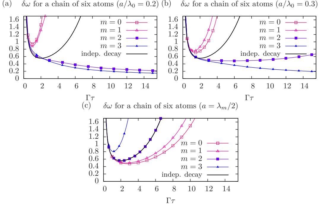
Figure 7.4: Numerical investigations for a 1D chain of six atoms Numerical results for the sensitivity as a function of \tau for a 1D chain of six atoms separated by a = 0.2\lambda_0 in a), by a = 0.3\lambda_0 in b) and by half of the magic wavelength in c). The different curves correspond to independent decay (solid line), SRT with m = 0 (empty squares) and PRT with m = 1 (empty triangles), m = 2 (filled squares) and m = 3 (filled triangles). In c) the independent decay overlaps with the curve for m = 2 .
