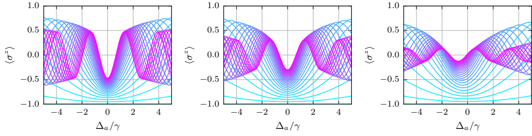
Figure 11.7: Simulated idealized Ramsey spectroscopy for different sets of effective cooperative interaction strengths, from left to right: subradiant case without shift ( \Omega^{\text{eff}} = 0, \Gamma^{\text{eff}} = -0.75 ), independent atom limit ( \Omega^{\text{eff}} = 0, \Gamma^{\text{eff}} = 0 ) and superradiant case with shift ( \Omega^{\text{eff}} = 1, \Gamma^{\text{eff}} = 1 ). The colours indicate the free evolution time with cyan representing a very short time and magenta meaning times up to 2.5\gamma^{-1} .
