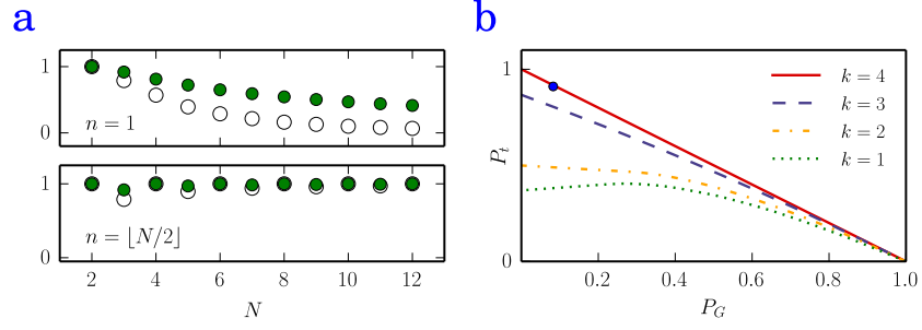
Figure 8.3: Entanglement properties. a) Comparison of the numerically computed von Neumann entropy (empty circles) of the reduced density matrix of the chain minimized over the atom index and the analytical expression for the entropy of the Dicke state (green circles), both for excitations n = 1 and n = \lfloor N/2 \rfloor as a function of the atom number N at distance a = 0.1\lambda_0 . b) Depth of entanglement of the subradiant four-atom state (blue dot) prepared by the magnetic field gradient scheme (see fig. 8.2e). It clearly lies above the k = 3 boundary indicating four-atom entanglement. The k -atom entanglement boundaries of the target state population P_t as a function of the ground state population P_G have been computed for the corresponding target state of a four-atom chain at distance a = 0.025\lambda_0 .
