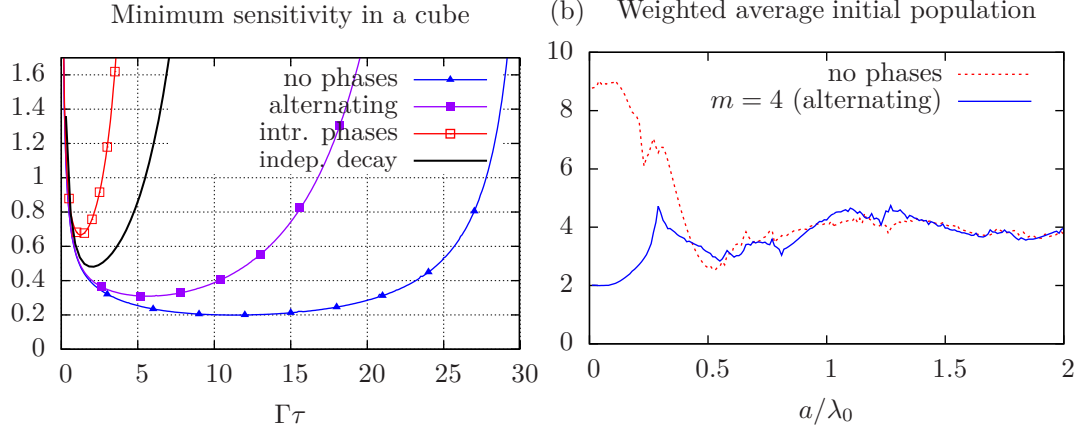
Figure 7.7: Numerical investigations for the cube configuration. a) Frequency sensitivity for the cube configuration in a magic wavelength lattice. b) Weighed average of decay rates with corresponding populations for SRT compared to PRT as a function of interatomic distance in a cube. As obvious from the plot, PRT outperforms SRT for distances roughly less than \lambda_0/2 .
