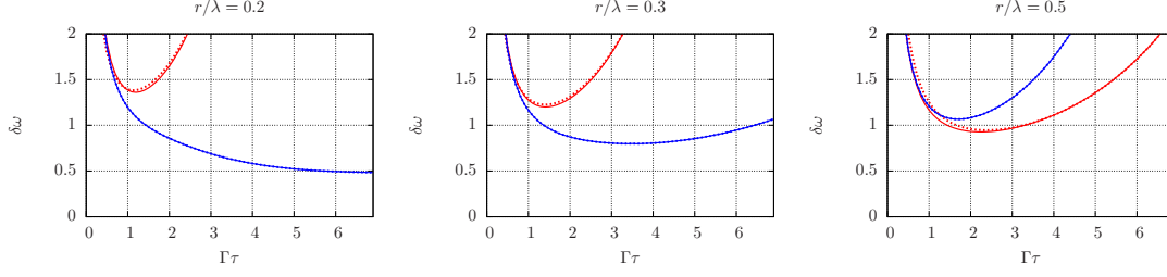
Figure 6.4: Analytical expressions (dashed) and numerical results (solid) for both the symmetric and asymmetric Ramsey procedures are compared showing almost perfect agreement (up to the small oscillations terms ignored in the derivation). Three distances have been chosen: r/\lambda = 0.2, 0.3 and 0.5 .
