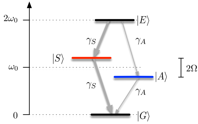
Figure 4.5: Super- and subradiance in two atoms. The symmetric state |S\rangle and the asymmetric state |A\rangle are shifted from the bare atomic energy by \pm\Omega . There are two non-interacting decay channels: the superradiant one involving the symmetric state with the rate \gamma_S = \Gamma + \gamma and the subradiant one with \gamma_A = \Gamma + \gamma involving the asymmetric state.
