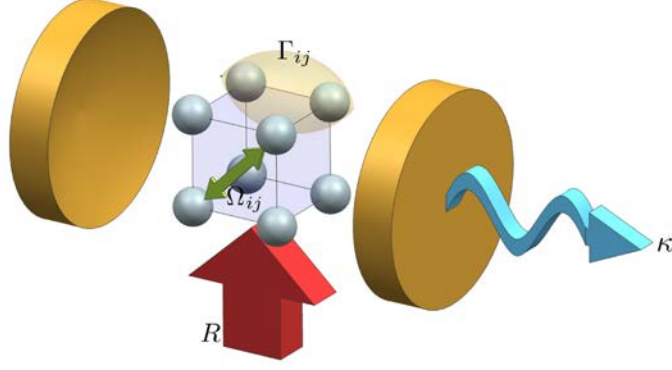
Figure 9.1: Schematics of a lattice laser setup. A transversely pumped (pumping rate R ) finite atomic ensemble with dipole-dipole couplings \Omega_{ij} and collective spontaneous emission \Gamma_{ij} inside an optical resonator with a loss rate of \kappa .
