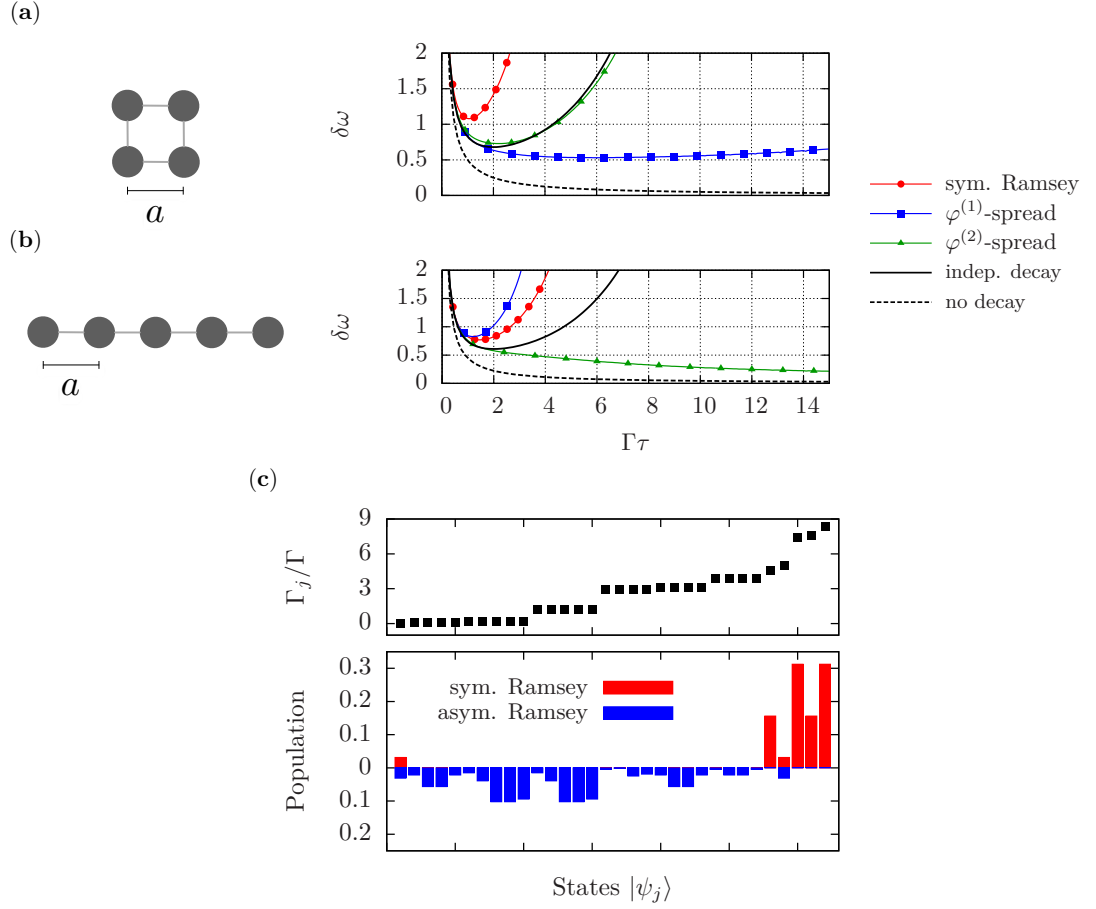
Figure 6.3: Numerical investigations. a) and b) Numerical results for the square and a 5 atom-chain. c) Results of diagonalization for an ideal system of 5 equally mutually coupled emitters. The states are ordered with increasing effective decay rate. The occupancy is shown in the histograms for symmetric vs. asymmetric Ramsey sequences.
