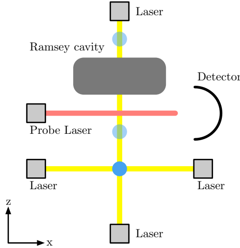
Figure 3.2: Schematic of a Fountain Clock Setup (y-dimension omitted). The atoms are laser-cooled in an optical molasses, then launched upwards and pass through the Ramsey cavity before they fall down again due to gravity and pass through the cavity a second time. They are then optically detected by a probe laser and a detector.
